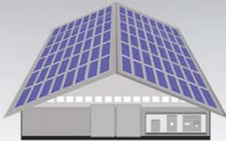
SOLAR SYSTEM
