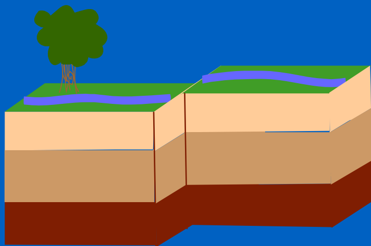
Strike-Slip
